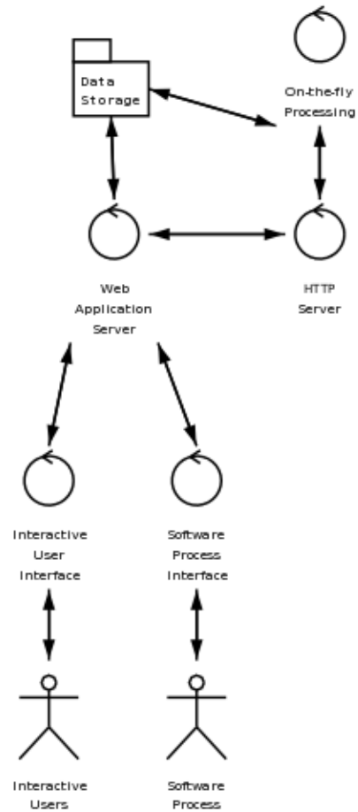
Figure 6.10. Live Access Server decomposed. Note that “Historical Database” is part of “Data Storage”
