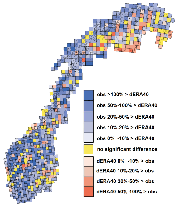
(b) Spring; max blue: OBS 251% > dERA40, max red: dERA40 89% > obs.
