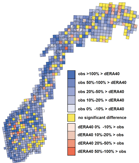
(c) Summer; max blue: OBS 241% > dERA40, max red: dERA40 90% > obs.
