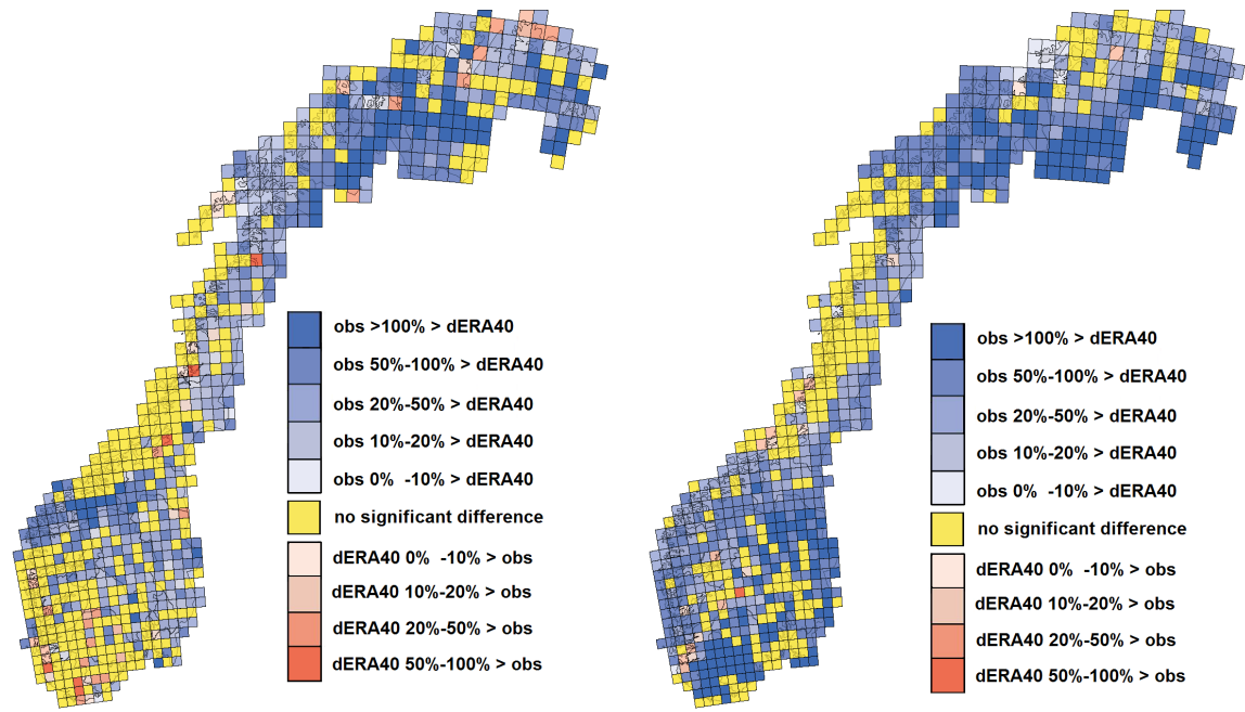
(a) Winter; max blue: OBS 300% > dERA40, max red: dERA40 84% > obs.
