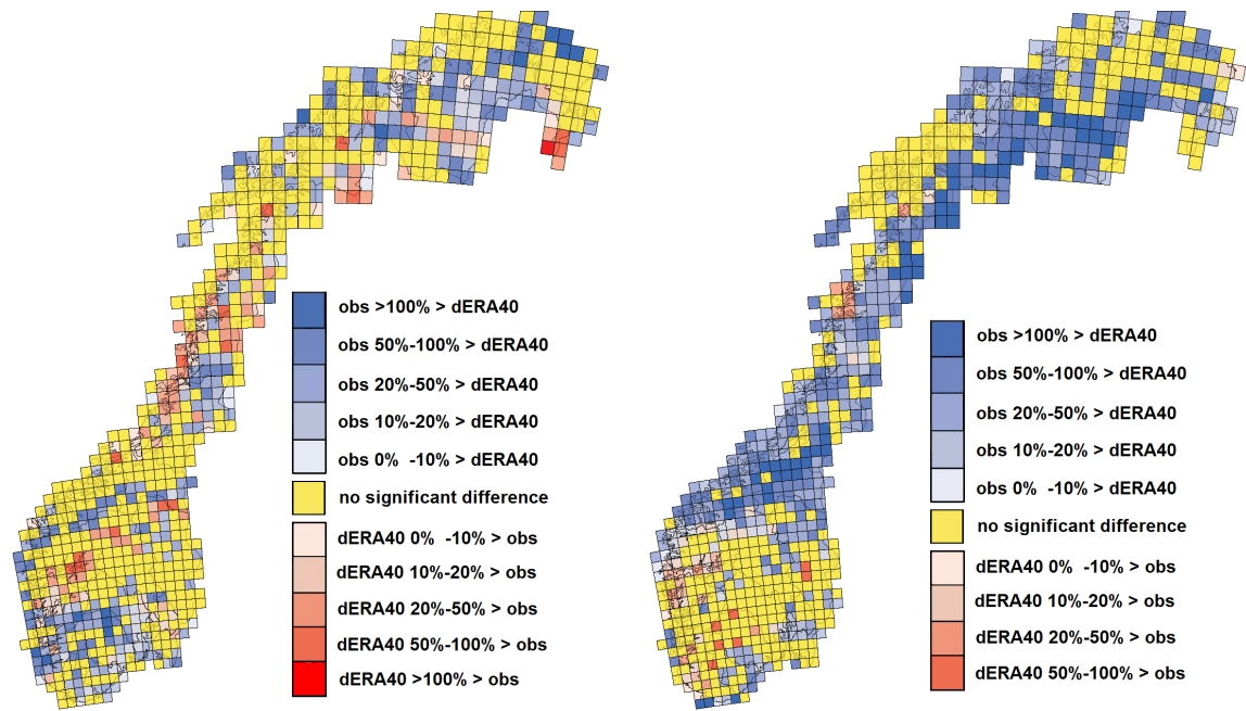
(c) Summer; max blue: OBS 192% > dERA40, max red: dERA40 118% > obs.
