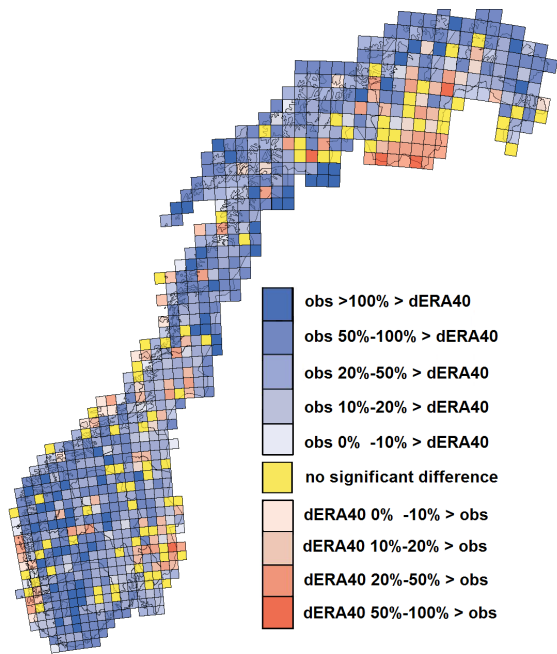
(a) Winter; max blue: OBS 384% > dERA40, max red: dERA40 84% > obs.
