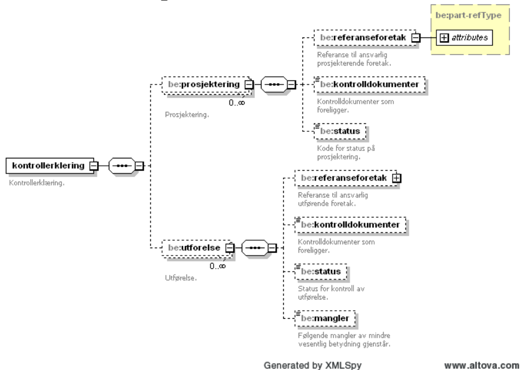
Figure 7 The kontrollerklæring XML structure in version 1.2
