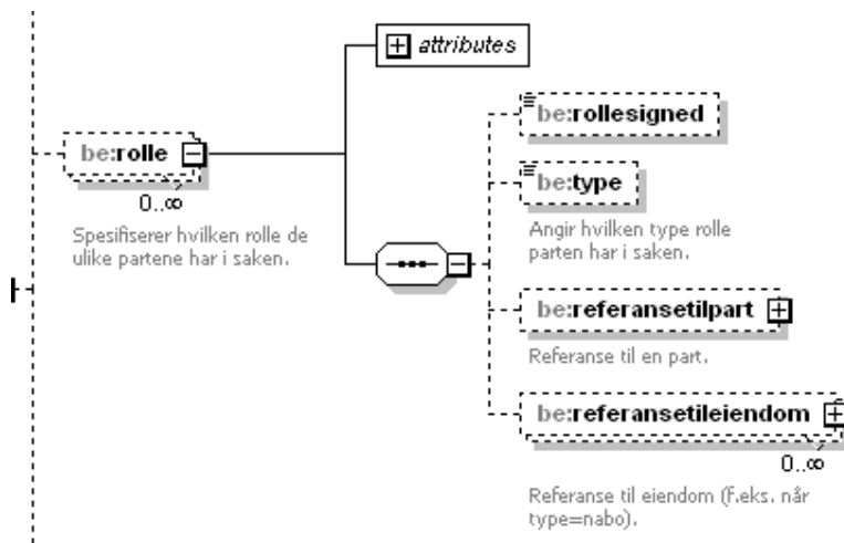
Figure 4 The rolle XML structure in version 1.2
