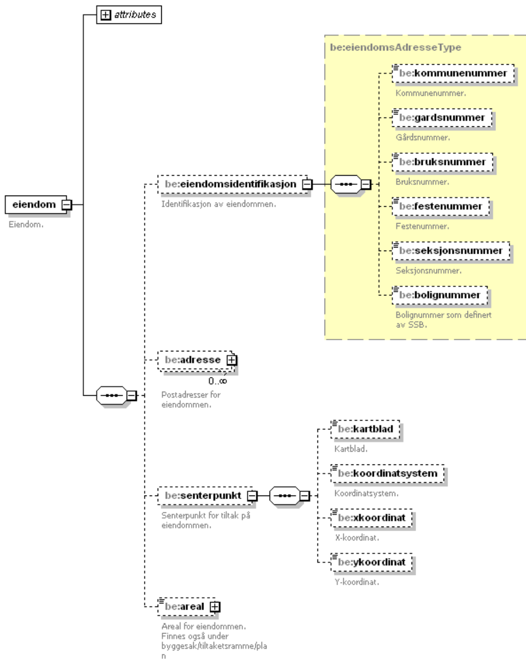
Figure 5 The eiendom XML structure in version 1.2
