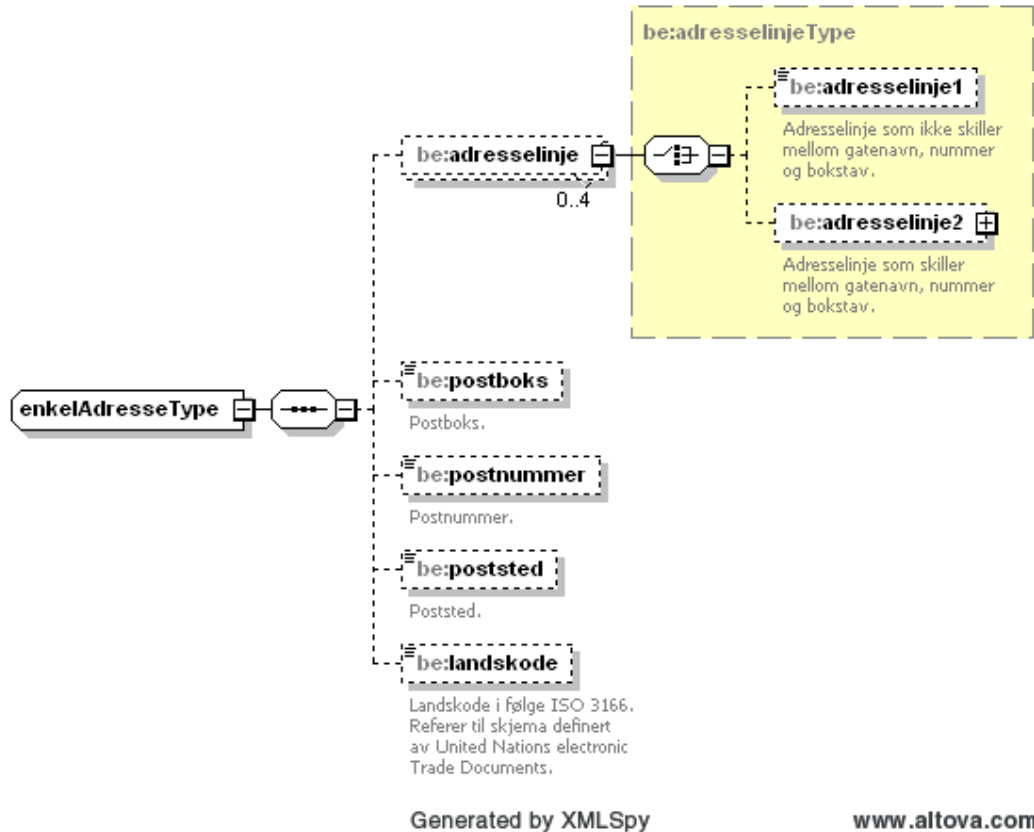
Figure 3 The enkelAdresseType XML structure in version 1.2
