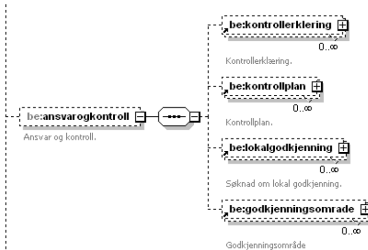
Figure 6 The ansvarogkontroll XML structure in version 1.2
