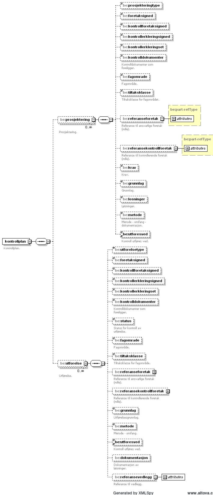
Figure 8 The kontrollplan XML structure in version 1.2
