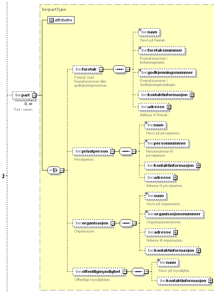
Figure 2 The part XML structure in version 1.2
