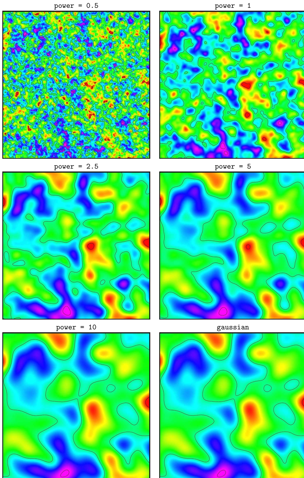
Figure 20.3. Rational quadratic variograms. Note that these variograms approach the gaussian variogram when power becomes large. This variogram is not numerically stable for large values of power so we recommend to use the gaussian variogram instead for power > 10.
