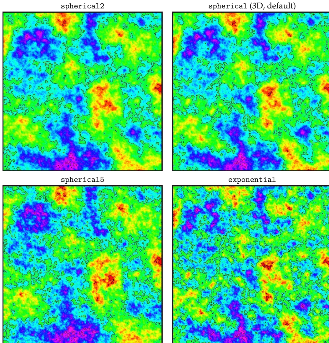
Figure 20.1. Spherical and exponential variograms.
