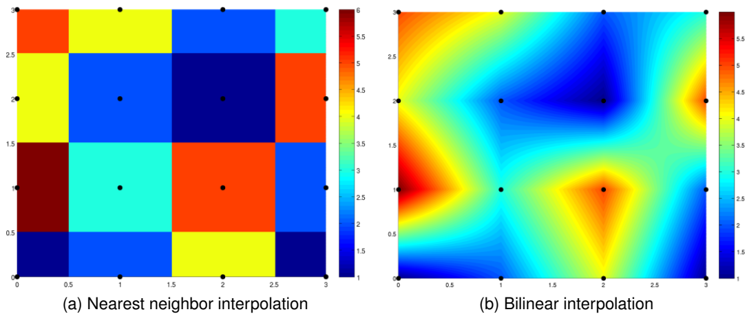
Figure 18.3. The images show how interpolation is applied to a series of data points (black dots) in the box [0, 3] \times [0, 3] . Pictures are taken from www.codecogs.com .
