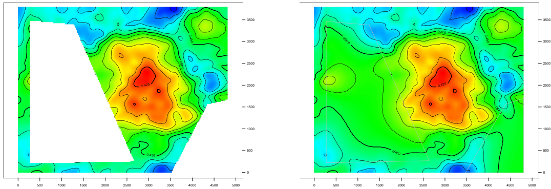
Figure 15.2. Original travel time map to the left with missing areas. Extrapolated travel time map to the right. The default extrapolation method (kriging with 1000 m range) has been used.
