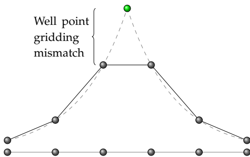
Figure 18.1. Vertical cross section of a surface. Grid nodes are marked as grey dots. A single well point is marked as a green dot. The dotted line is the kriging predictor and the solid line is the bilinear interpolation between the grid nodes. The gridding error is the vertical difference between the dashed line (kriging) and the solid line segments (bilinear interpolation). The gridding mismatch at a well point is the vertical difference between the green dot and the solid line connecting the two nearest grid nodes.
