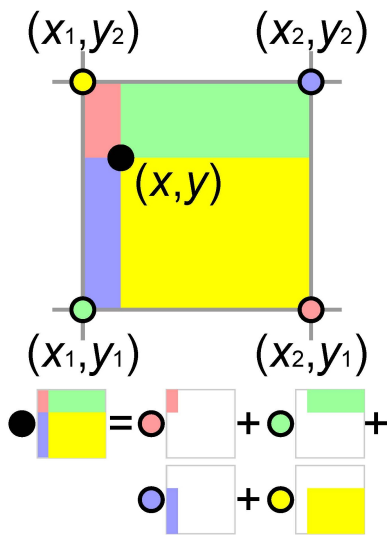
Figure 18.2. Illustration of bilinear interpolation. The value at the black dot, (x, y) , is the weighted average of the values at the colored dots, (x_i, y_j) ; i, j = 1, 2 , where the weights are proportional to the area of the rectangle of the same color. The illustration is taken from Wikipedia .
