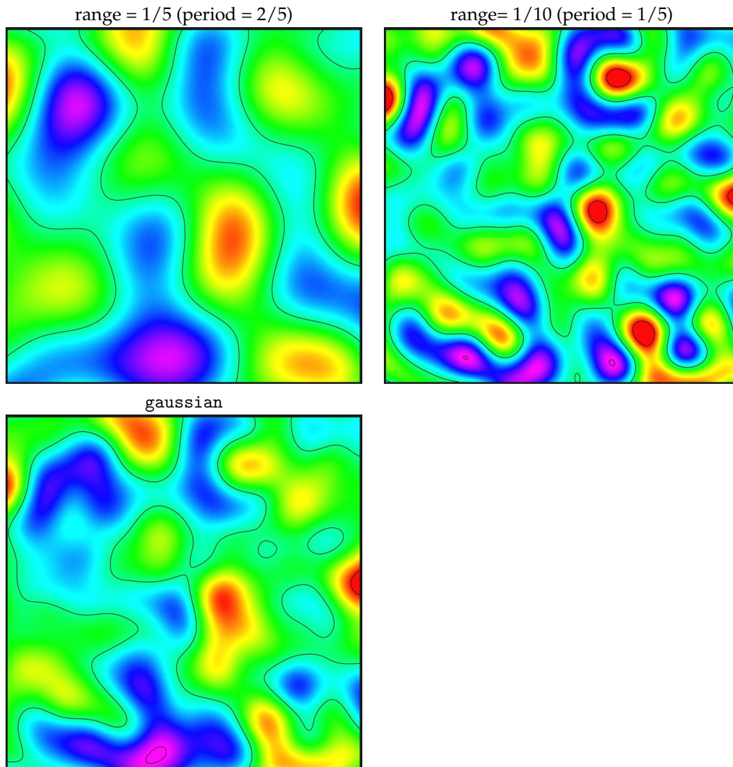
Figure 20.4. Damped sine variograms. The damped sine variogram gives a smooth regular cyclic appearance. The full period is twice the specified range. The gaussian variogram is added for comparison.
