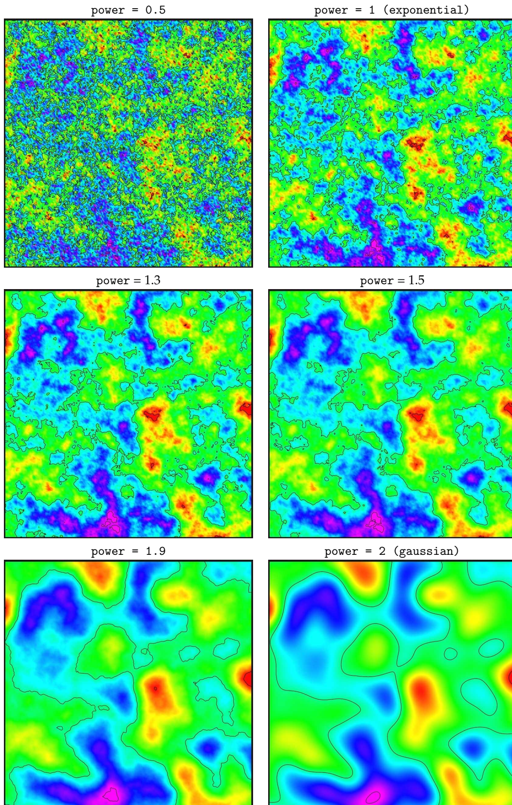
Figure 20.2. General exponential variograms for different <power>. Note that the exponential variogram is identical to power = 1 and the gaussian variogram is identical to power = 2.
