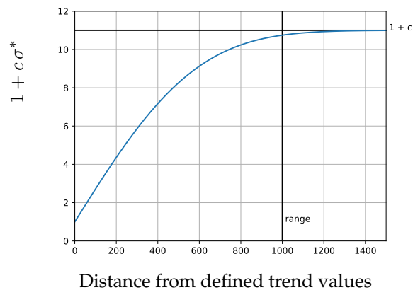
Figure 15.3. Increase in residual SD in areas with extrapolated trend maps. The default value c = 10 is used in the figure. The SD increases until it reaches the range given by <extrapolation-kriging-range> where it flattens at 1 + c times the original local SD value. The factor c is specified by <extrapolation-SD-factor>.
