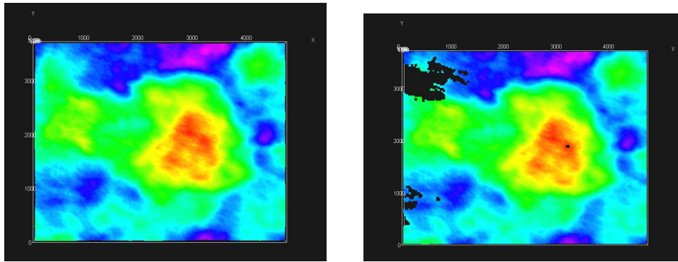
Figure 15.4. Original surface to the left (default). To the right is <set-eroded-nodes-to-undefined> set to yes.
