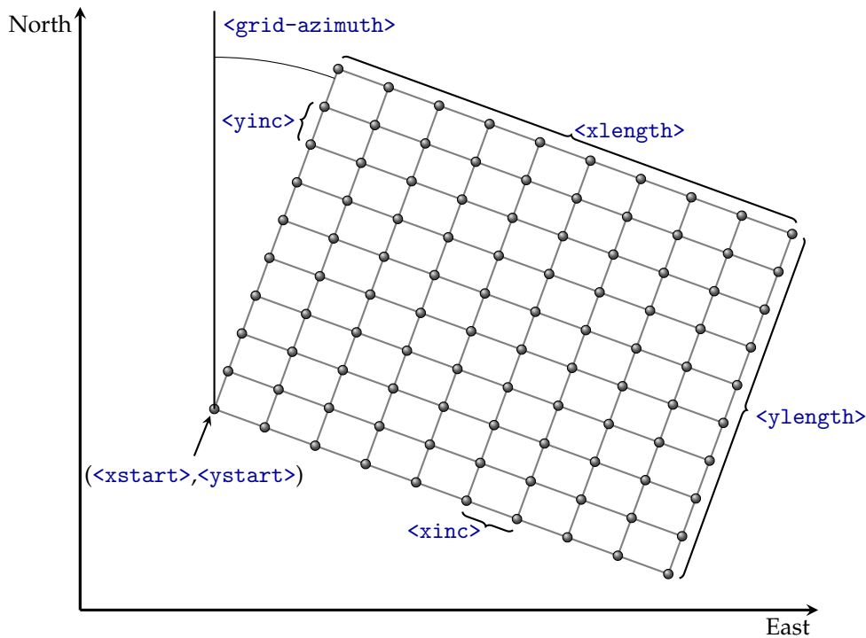
Figure 15.1. Elements used to specify the output grid definition: <grid-azimuth> , <xinc> , <yinc> , <xlength> , <ylength> , <xstart> and <ystart> . Note that using <read-from-file> is simpler. The surfaces are defined at the grid nodes (gray bullets). COHIBA uses bilinear interpolation (Section 18.6.1) to approximate the surfaces inside the rectangles.
