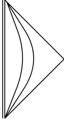
Figure 18: Penrose–Carter diagram in the (z, t) plane for an extreme Type I dilatonic domain wall with \alpha > 1 . The arcs correspond to the wall separating the semi-infinite Minkowski space–time and the space–time with a varying dilaton field and the naked planar singularity (the double line).
