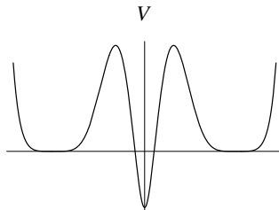
Figure 24: Modular invariant potential along the geodesic T(z) = e^{i\Phi(z)} for the Kähler potential and superpotential of Eq. (8.8).
